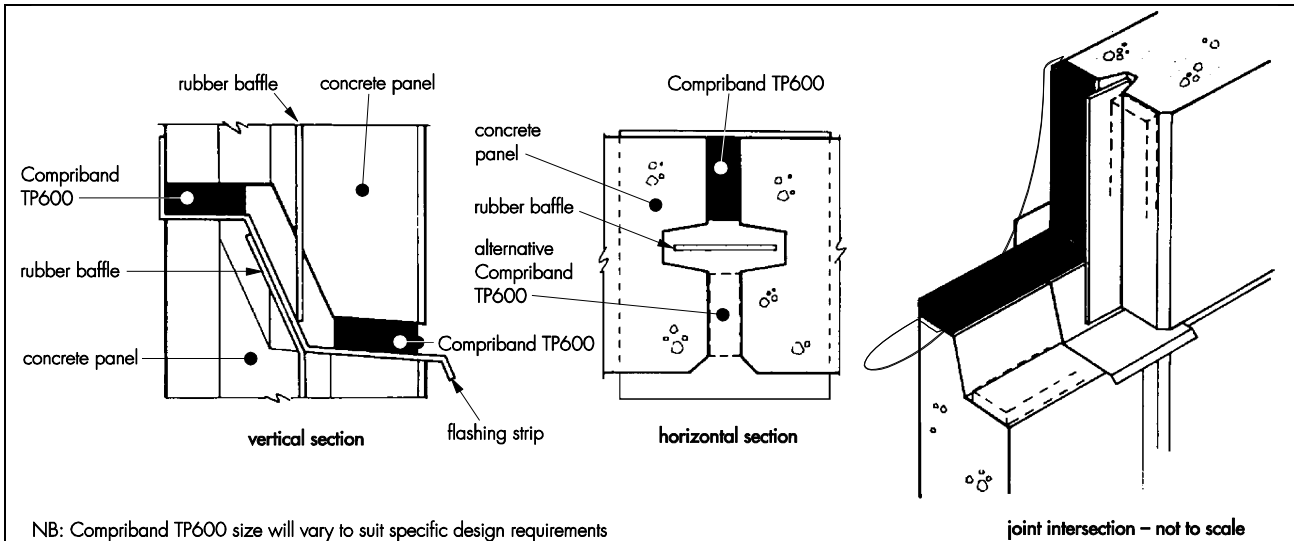
Figure 2 Walls — precast concrete panels
