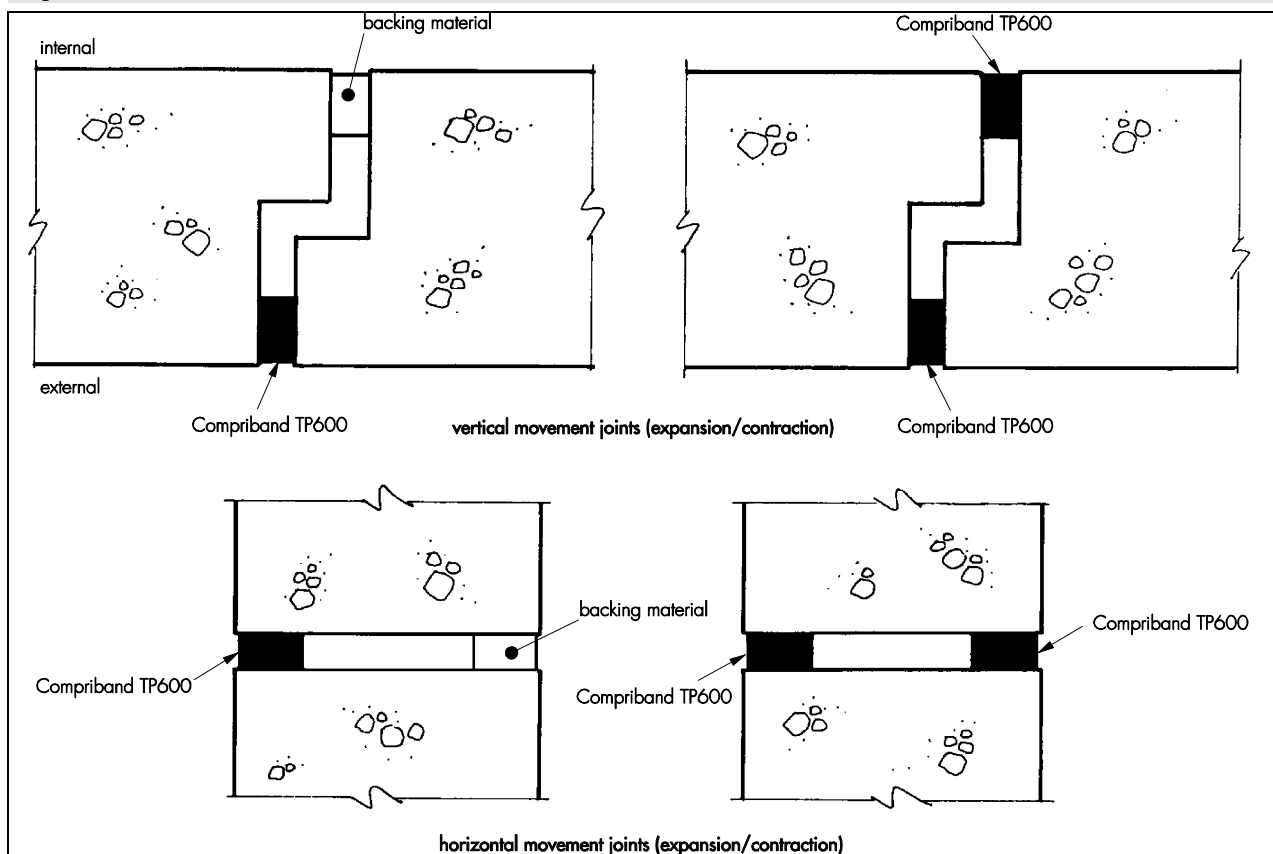
Figure 1 Walls
