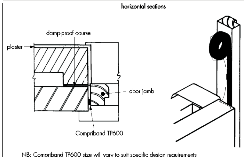
Figure 4 Door and window jambs — timber
