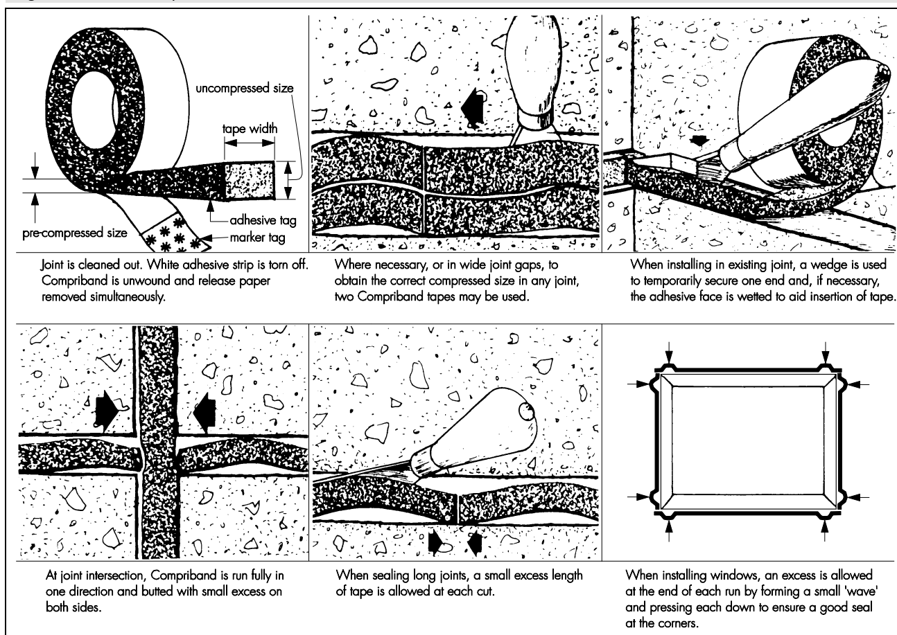
Figure 7 Installation practices
