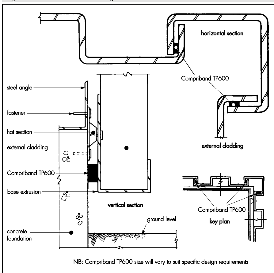
Figure 6 External sheet cladding
