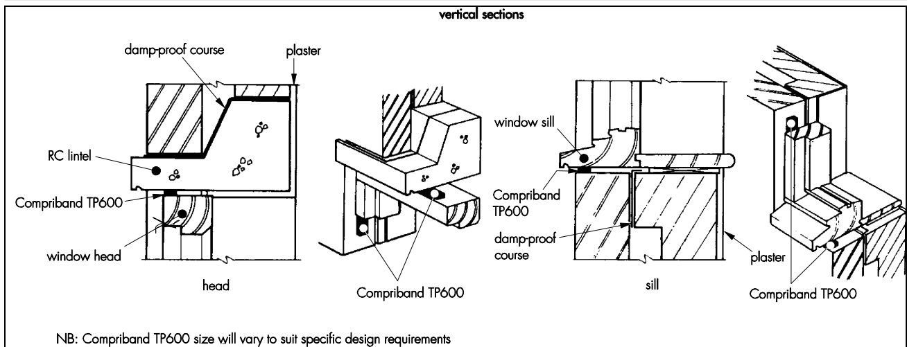
Figure 3 Door and window head and sills — timber
