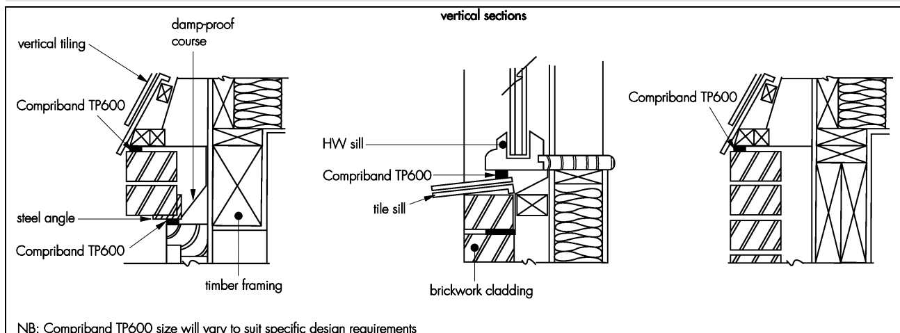
Figure 5 Timber frame walls
